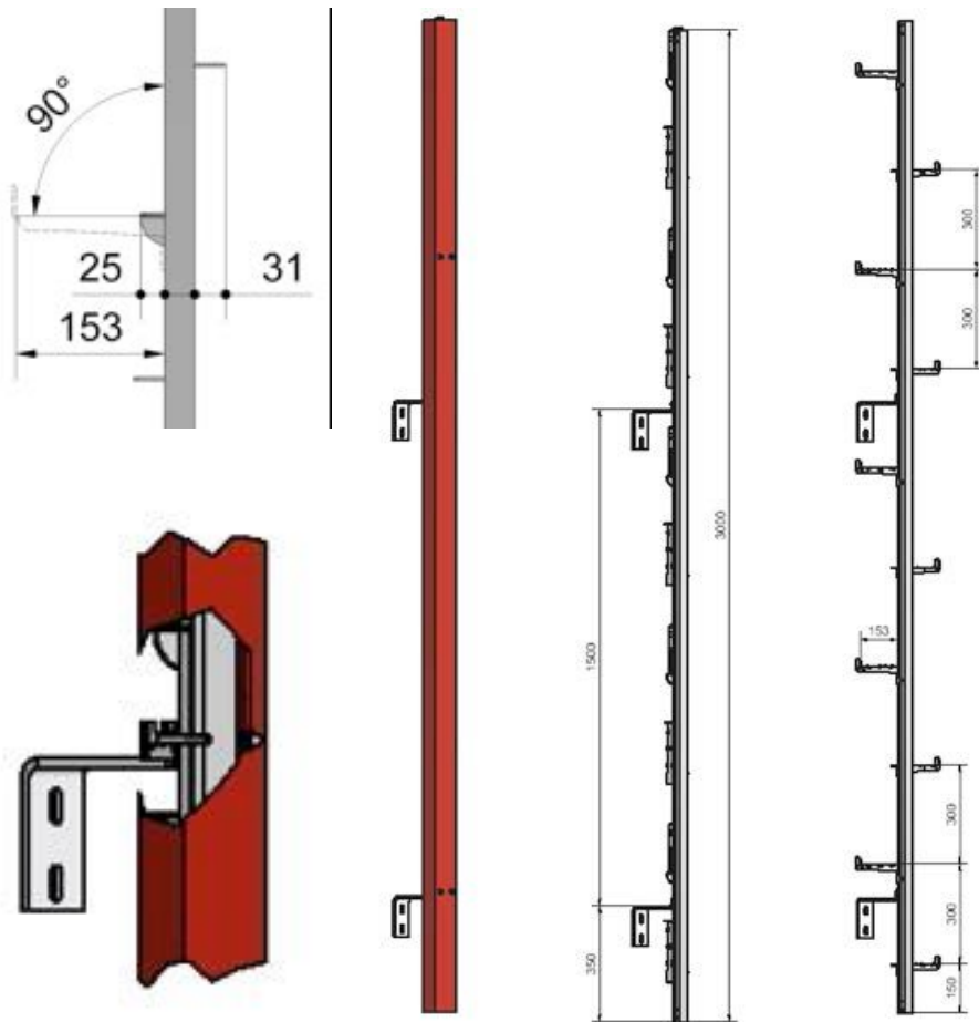
RHF030 out of/in service
